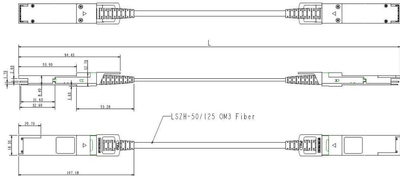
Figure8. Mechanical Specifications
